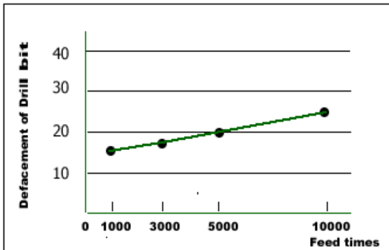
Drilling processability 钻孔加工性
