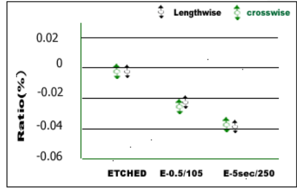
Dimensional stability-PCB process (size:360*310mm)
