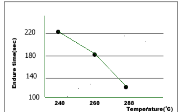
Solder Resistance 耐焊性
